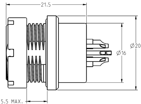
ER: Rear Panel Mount
