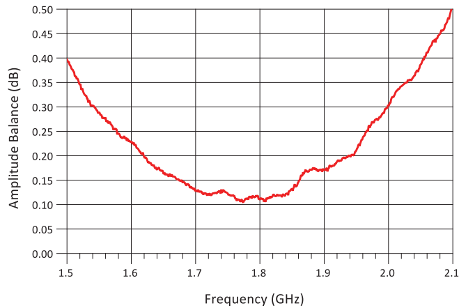
Amplitude Balance
