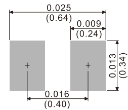
DFN0603-2L
