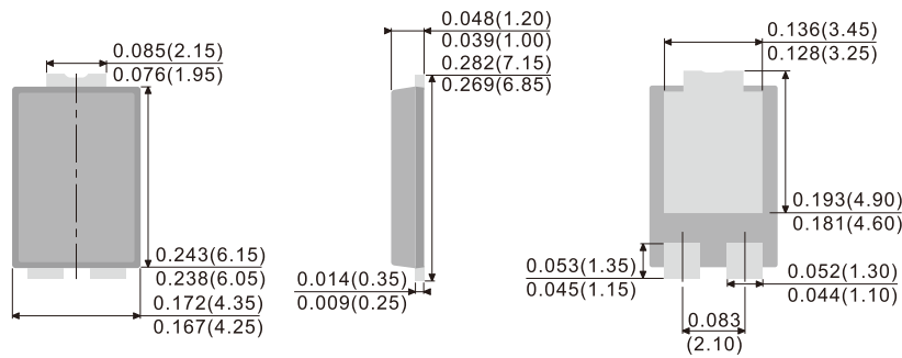
TO-277C
