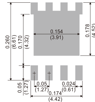
DFN5060B-8L
