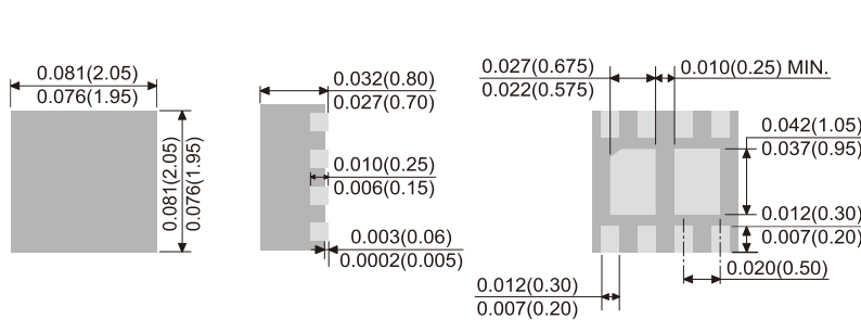
DFN2020-8L
