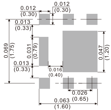
DFN2020-8L
