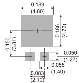
TO-277C
