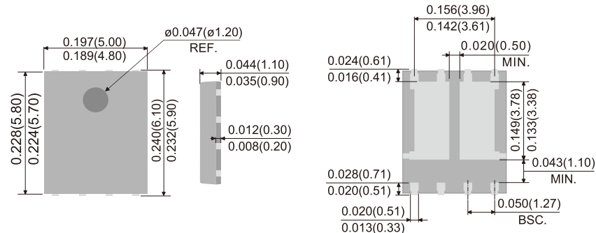
DFN5060B-8L
