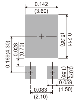
TO-277C
