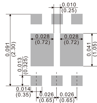
DFN2020B-6L
