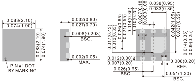
DFN2020-8L
