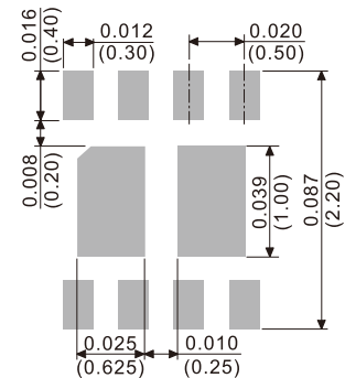
DFN2020-8L
