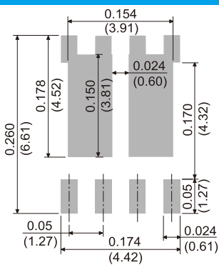
DFN5060B-8L
