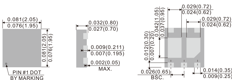
DFN2020-6L
