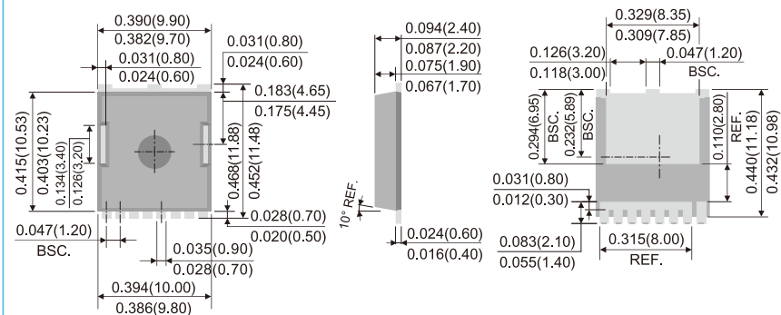
TO-LL
