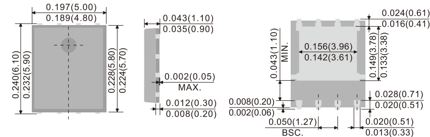
DFN5060B-8L
