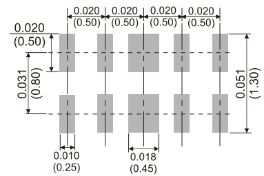
DFN2510A-10L
