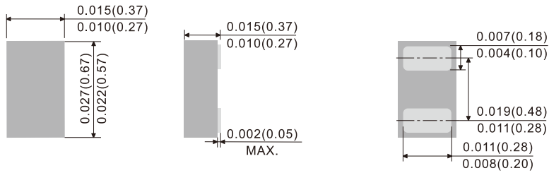
DFN0603-2L
