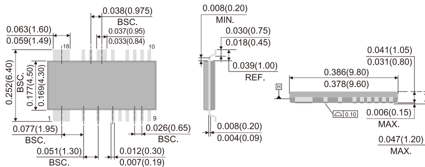
TSSOP-18
