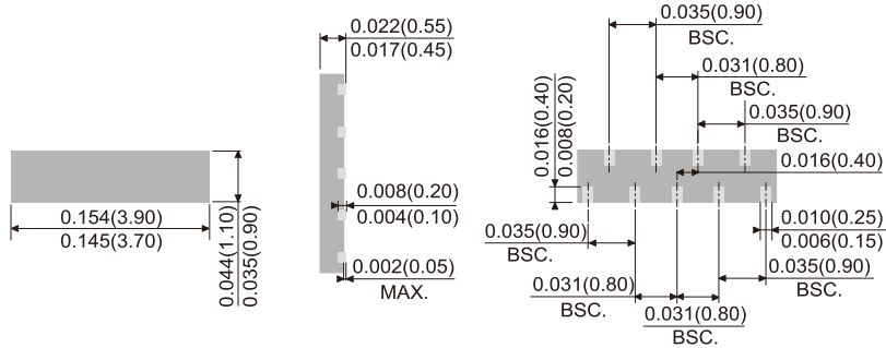
TO-LL
