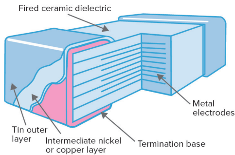
FlexiCap™ MLCC cross section
