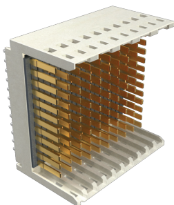
Vertical Header 2 Wall
