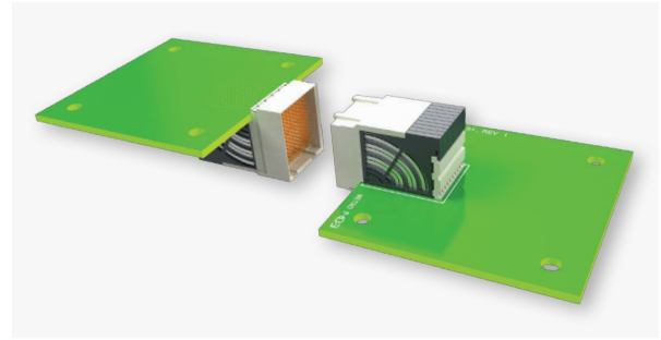
AirMax VS2® COPLANAR CONNECTORS – INVERSE
