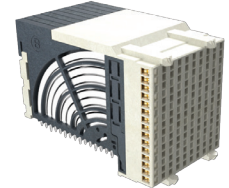
Right Angle Receptacle (No Guide)
