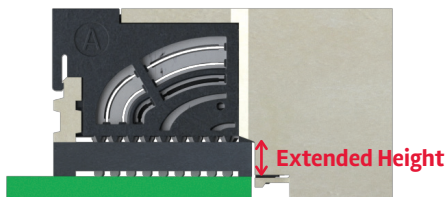
Pin-in-Paste PCB termination
